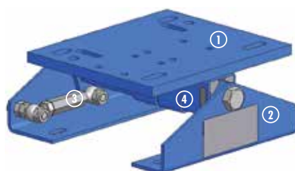
MB 27 x 120 Steel parts blue painted
